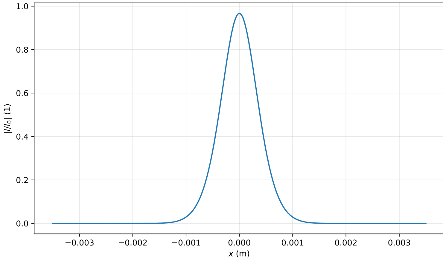
Intensity profile I(x, y = 0, z = 1.115m)/I_0 , P_{in}=0.4P_{cr} , artificial time
